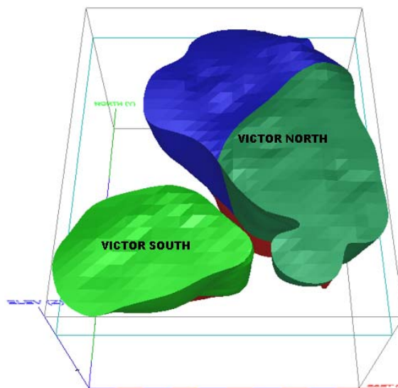
Figure 1: Victor South and Victor North kimberlite pipes. Green=pyroclastic kimberlite; blue=so-called hypabyssal kimberlite. Intervals on the east axis are 50m.
