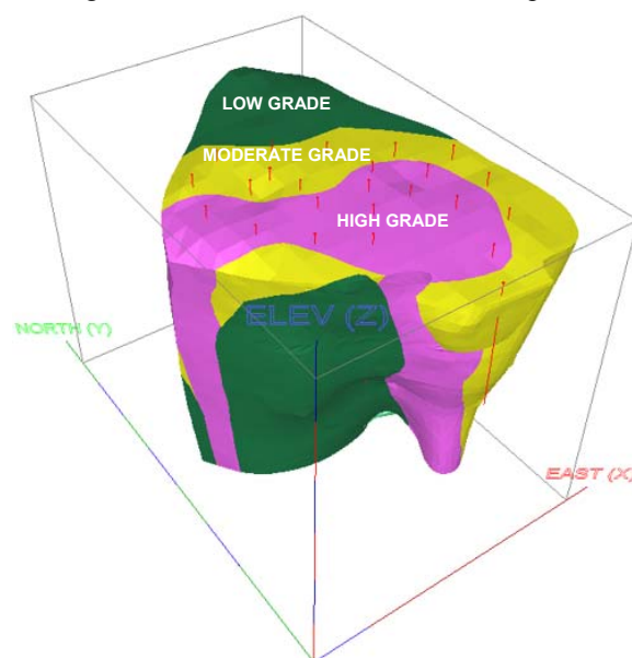
Figure 6: Macrodiamond sample grade distribution in Victor North PK (2001/2002 bulk sampling programme), courtesy of the Victor Project. Intervals on the vertical axis are 50m. Red markers indicate large diameter drillholes.
