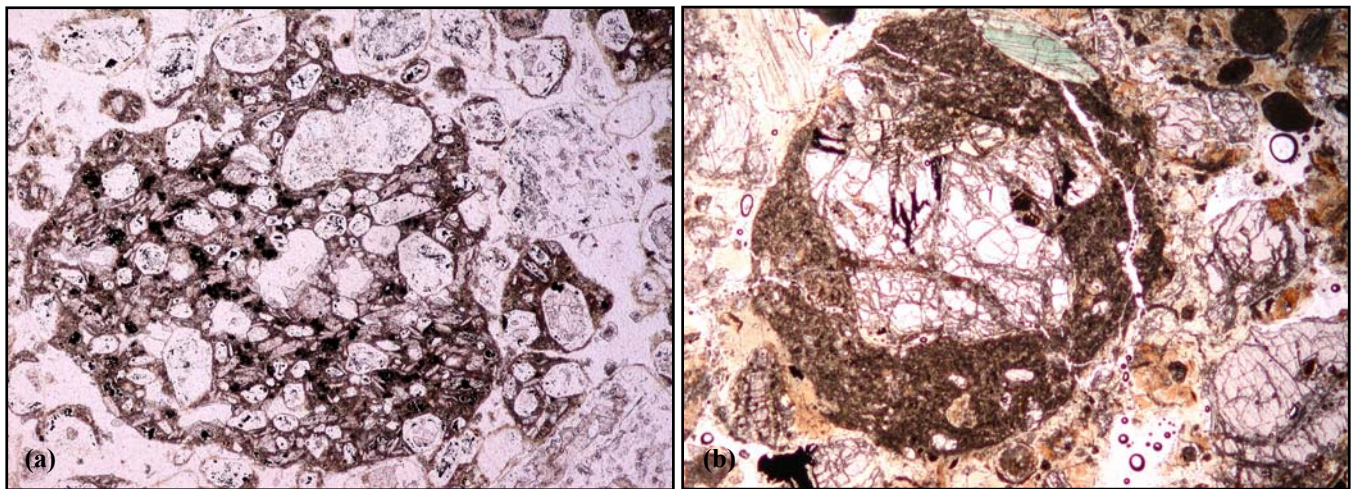
Figure 3: Photomicrographs of the (a) olivine phenocryst-rich pyroclastic kimberlite and (b) olivine phenocryst-poor pyroclastic kimberlite, showing the contrasting modal abundance, size and habit of the primary olivine phenocrysts that occur both within the juvenile lapilli and as discrete grains. PPL. FOV = (a) 3mm, (b) 8mm.
