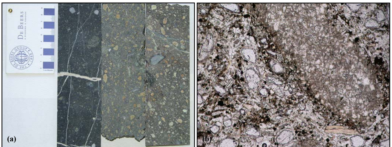
Figure 4: The dark competent so-called hypabyssal kimberlite shown in (a) polished drillcore and (b) thin section. The photomicrograph shows the unusual uniform to magmatic texture of these rocks. PPL. FOV = 6mm
