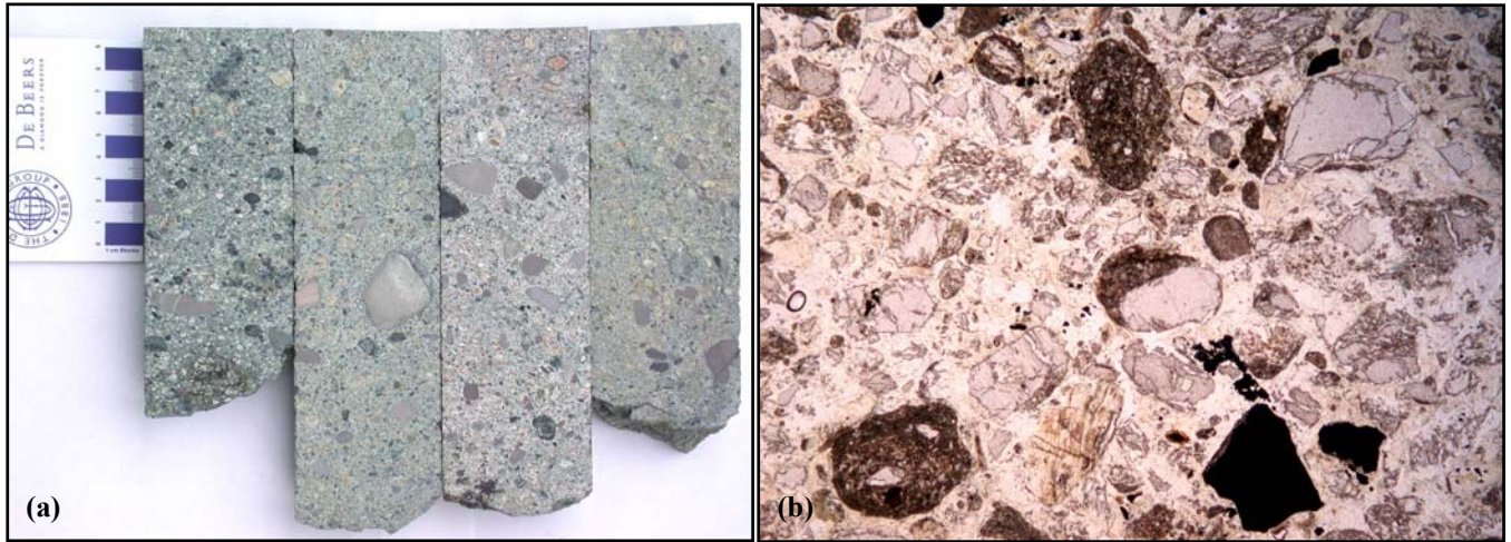
Figure 2: Typical Victor pyroclastic kimberlite shown in (a) polished drillcore and (b) thin section. The photomicrograph shows abundant clast supported discrete fresh and altered olivine and lesser subround juvenile lapilli set in a serpentine matrix. PPL. FOV = 9mm.
